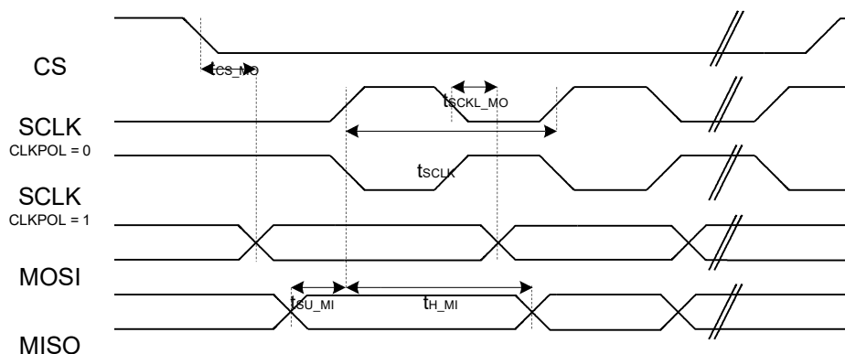
Figure 4.1. SPI Master Timing Diagram
