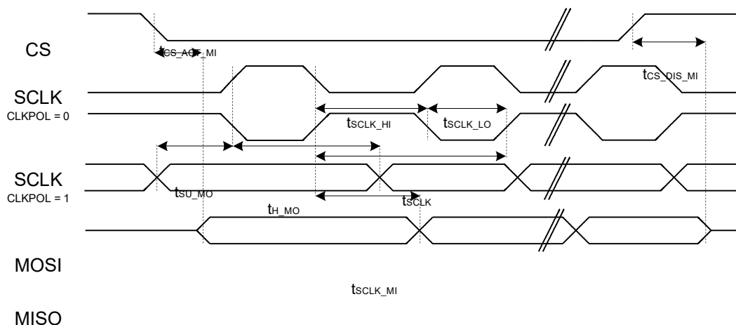
Figure 4.2. SPI Slave Timing Diagram
