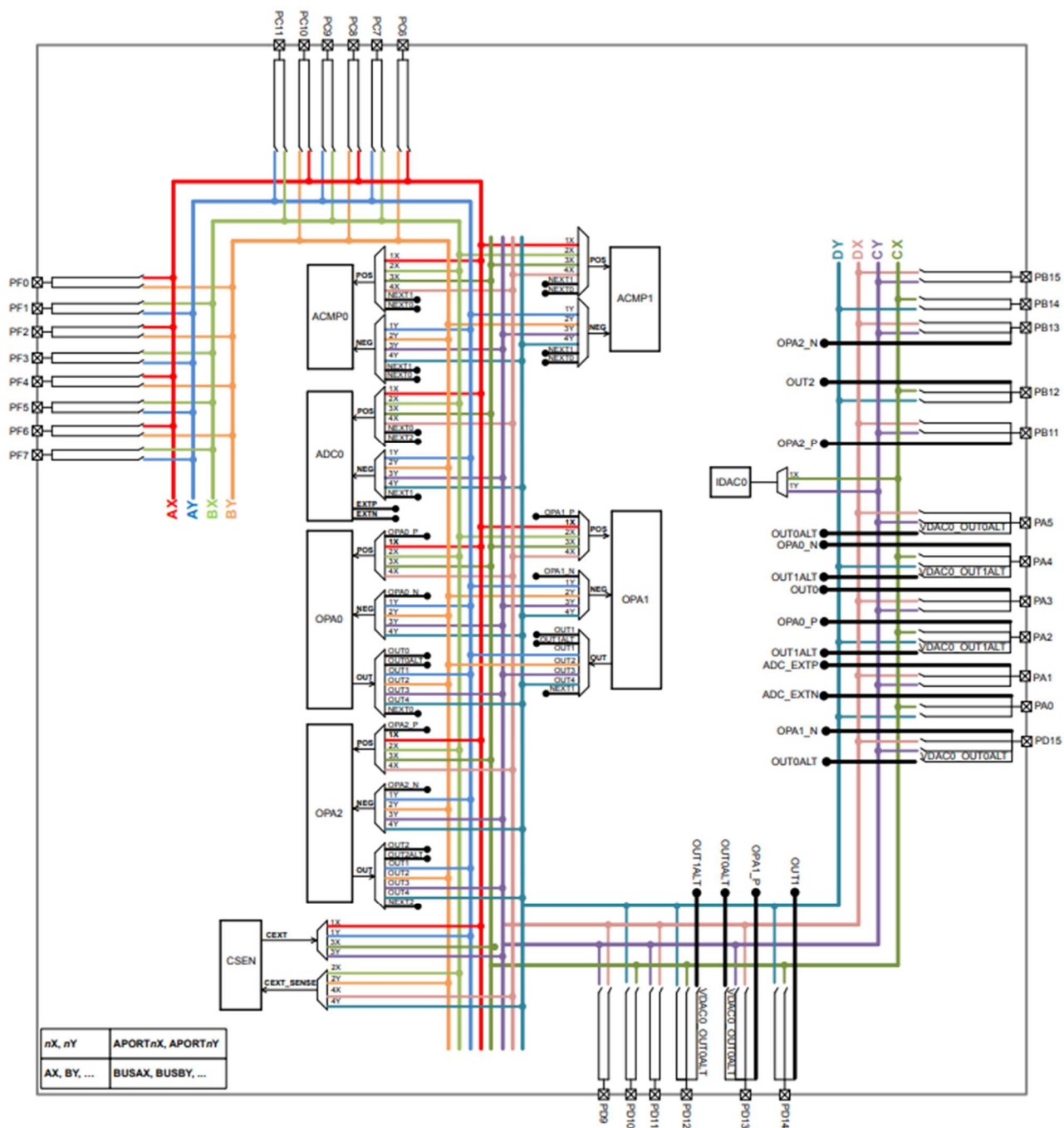
Figure 6.2. APORT Connection Diagram
