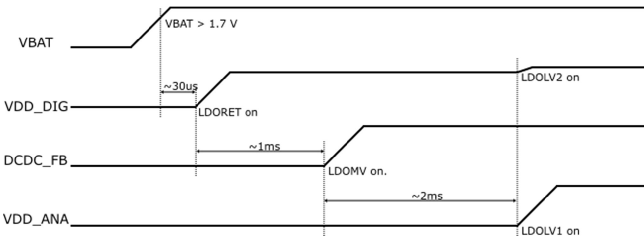
Figure 1.28-2 Power-on Sequence
