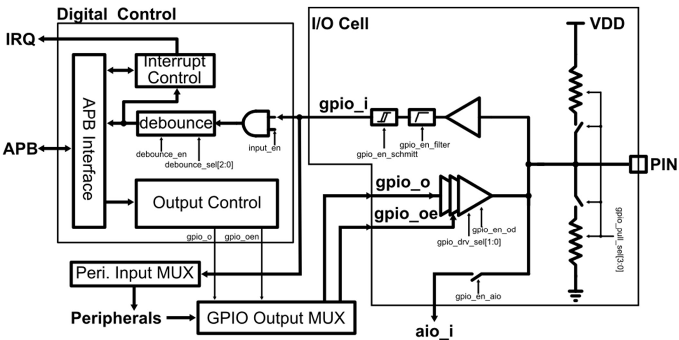
Figure 1.17-1 Block Diagram of GPIO
