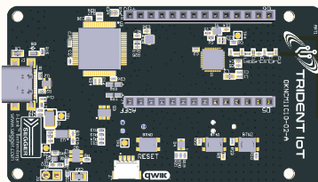
PCBDKNCM11C10-02
